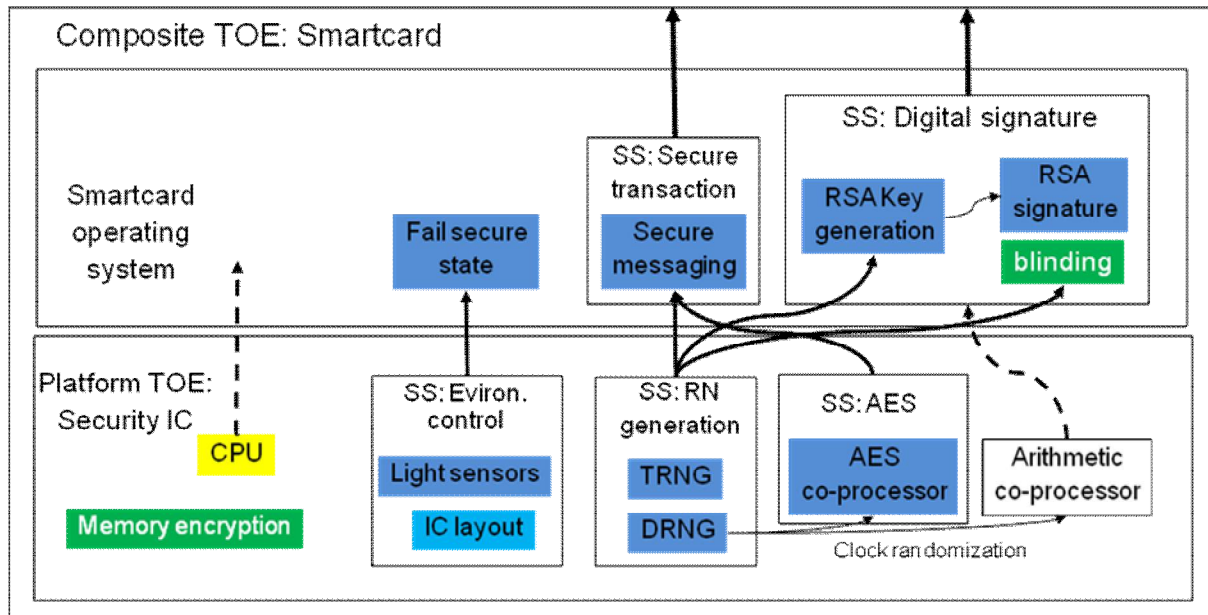
Figure2 Examples of security services, security functions, security mechanisms and architectural countermeasures
